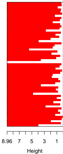
Banner of diana(x = dM) Dendrogram of diana(x = dMa)
