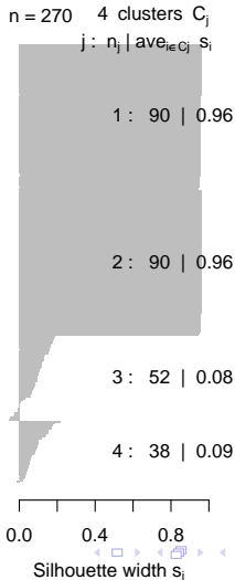
Silhouette plot of pam(x)
